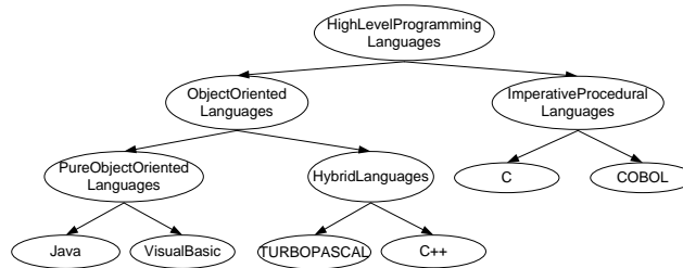
Fig. 2. Skills hierarchy
